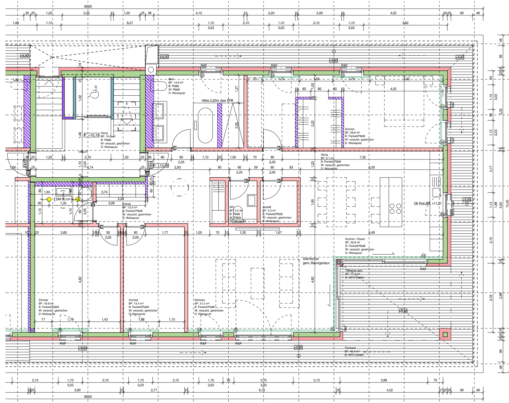
Grundriss Attika
